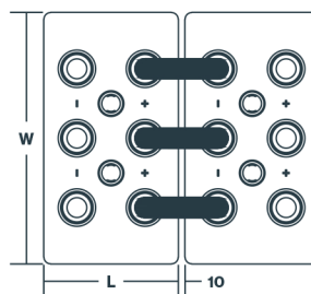
14 OPzS-ET2450SOLAR - 18 OPzS-ET3150SOLAR
