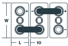
2 OPzS-ET160SOLAR - 7 OPzS-ET1070SOLAR
